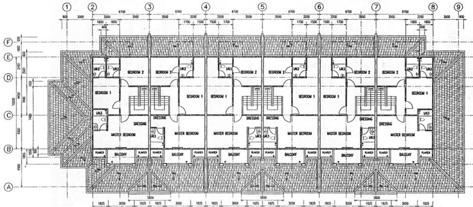
FIRST FLOOR PLAN ( S/L 1 TO 6 )
